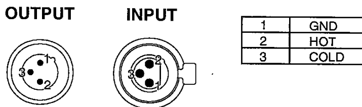
Figure 30 XLR wiring
