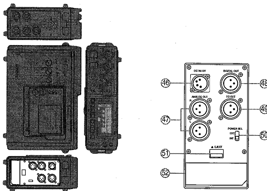
Figure 8 Output connectors
