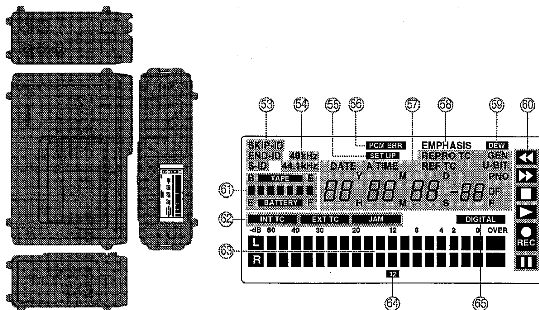
Figure 9 LCD panel
