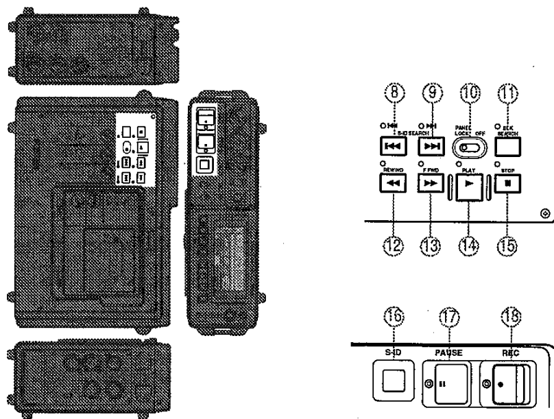
Figure 3 Transport controls
