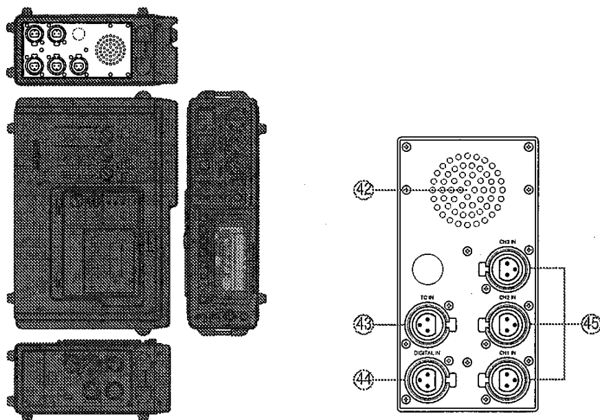
Figure 7 Input connectors
