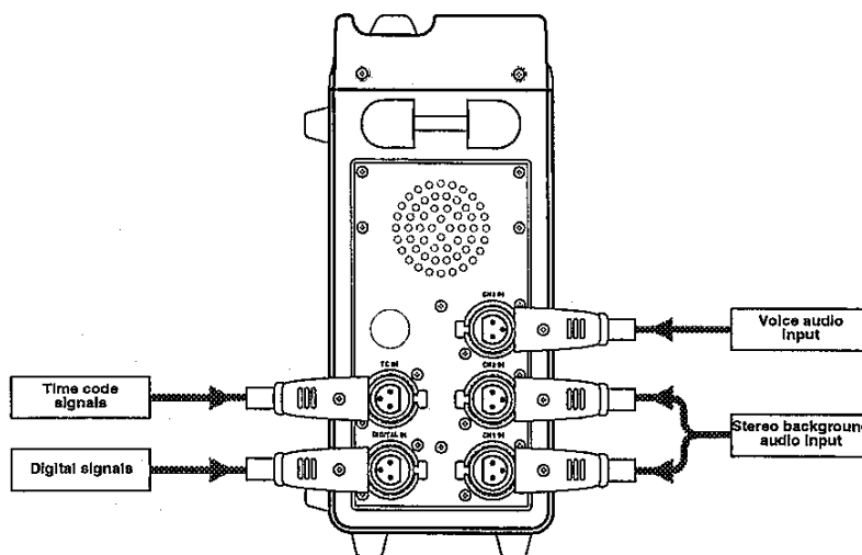
Figure 13 Input connections
