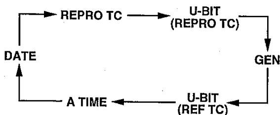
Figure 24 24H RUN mode
